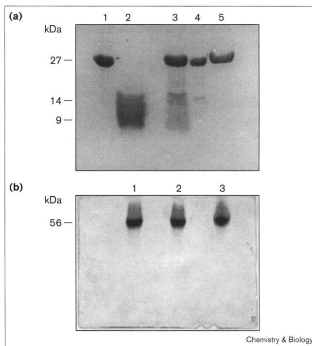
(a) SDS-PAGE analysis of PfTIM, subtilisin digest and religated products in various organic solvents. Lane 1, wild-type TIM migrating as a 27 kDa protein; lane 2, the subtilisin digest of wild-type TIM resulting in fragments that migrate at around 9–12 kDa; lanes 3, 4 and 5, the religation of the subtilisin generated fragments that yields a band co-migrating with native TIM in the organic solvents dioxan, 2,2,2-trifluoroethanol and acetonitrile, respectively. (b) Analysis of subtilisin-derived fragments and the religated TIM on a nondenaturing PAGE. Lane 1, native TIM; lane 2, the subtilisin digest; lane 3, the religated TIM in acetonitrile. It is important to note that TIM is a dimer and migrates as a ~56 kDa protein (dimer) under nondenaturing PAGE conditions.
